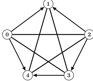
Figure 4: The directed graph \vec{A}_5^c (complement of \vec{A}_5 ). Bidirected edges are shown as undirected ones.
