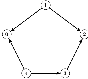
Figure 3: The directed graph \vec{A}_5 .
